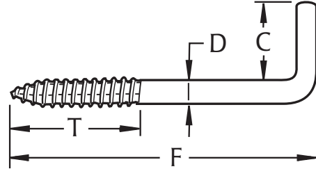
Screw Hook (Square Bend)
