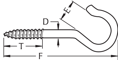
Screw Hook (Round Bend)
