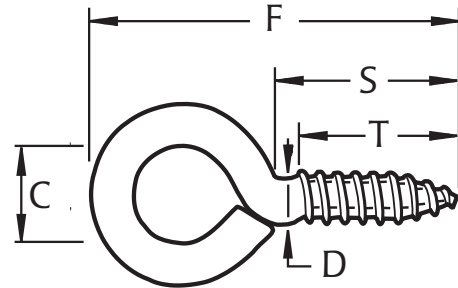
Screw Eye
