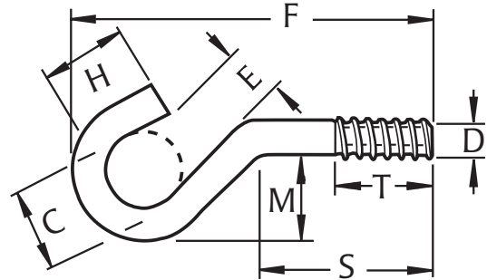
J-Bolt (Offset)
