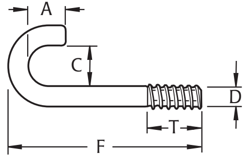
J-Bolt (Straight)
