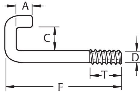
Hook Bolt (Square Bend)
