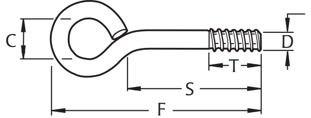
Eye Bolt (Closed)
