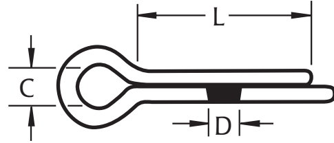
Cotter Pin (Standard)
